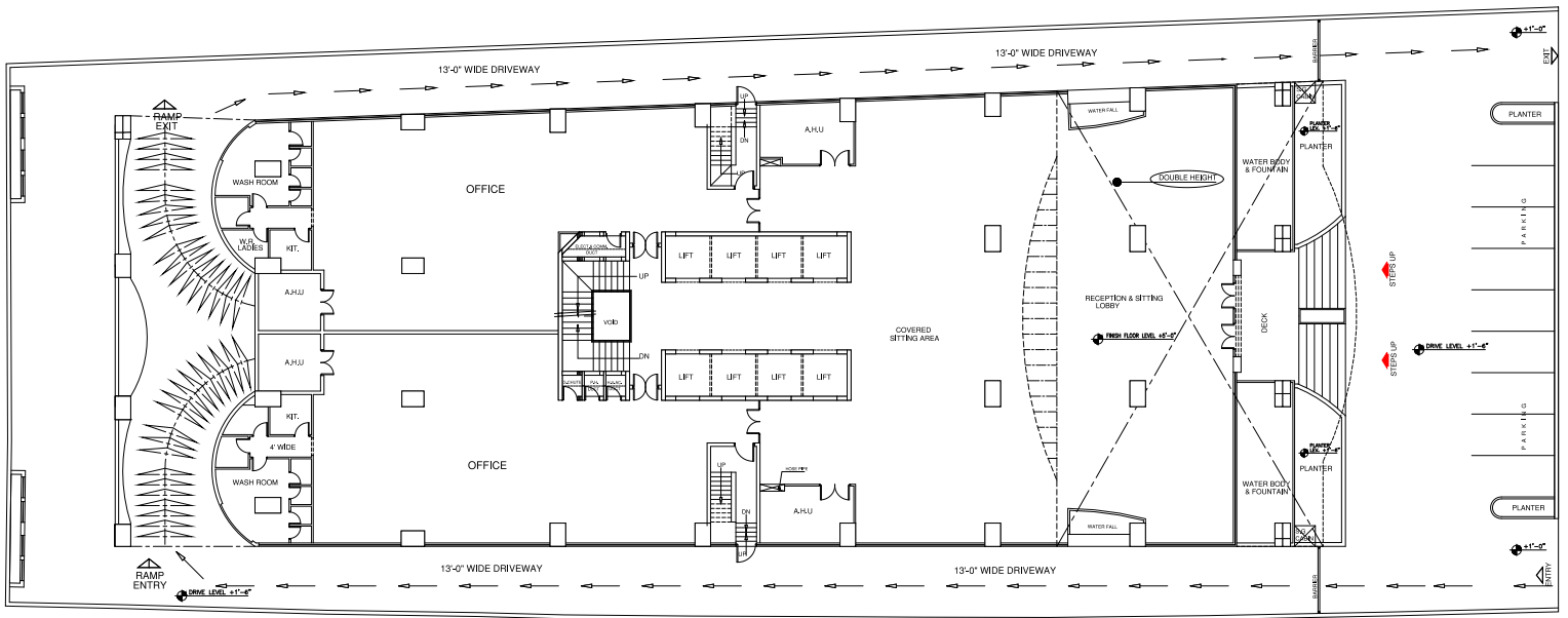
GROUND FLOOR PLAN RECEPTION & OFFICES NOS. OF CAR=9
