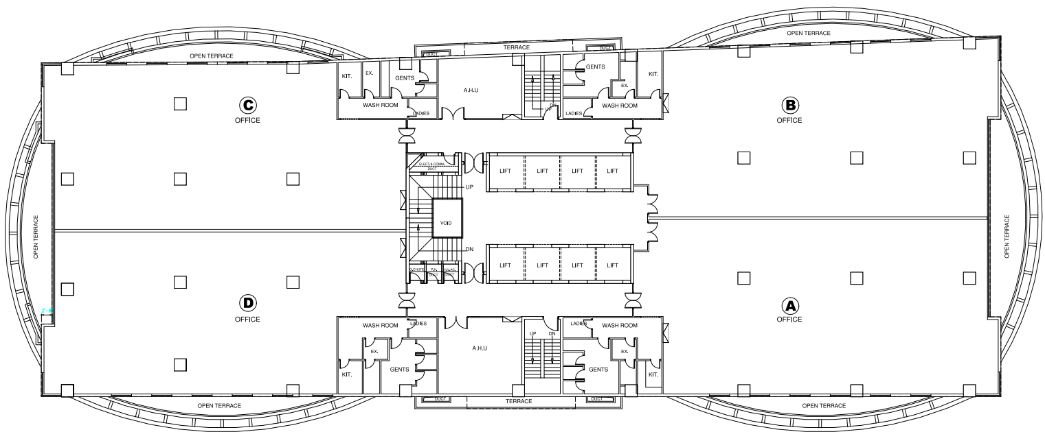
15th FLOOR PLAN OFFICES
